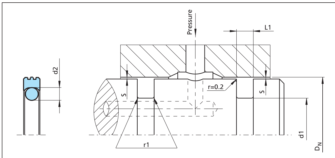
Figure 120 Installation drawing
