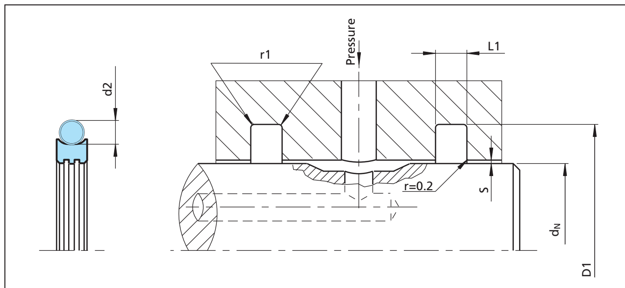
Figure 121 Installation drawing
