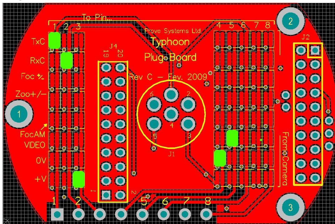
Tritech Waterblock - Serial Control
