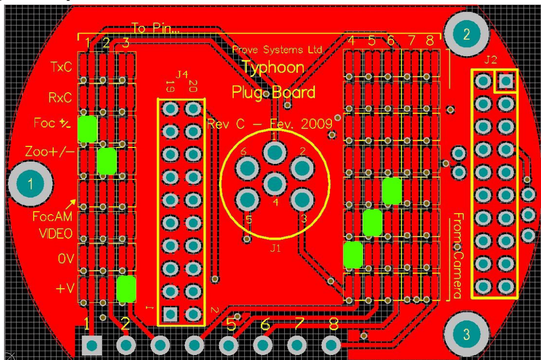
Tritech Waterblock - Analogue Control
